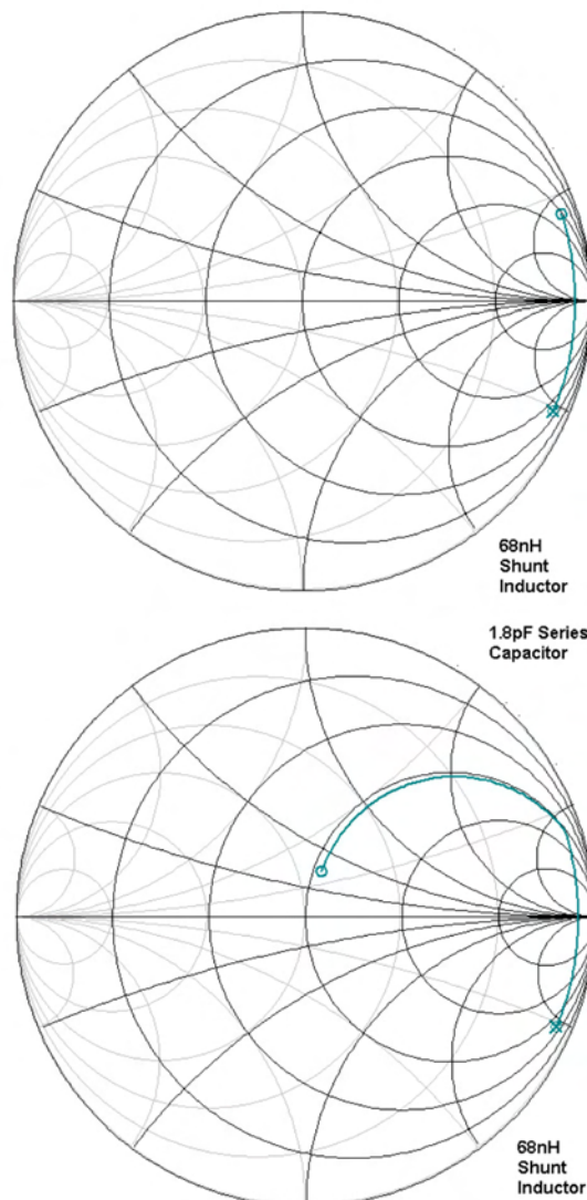
Figure 5. Plotting the Shunt Inductor and Series Capacitor
