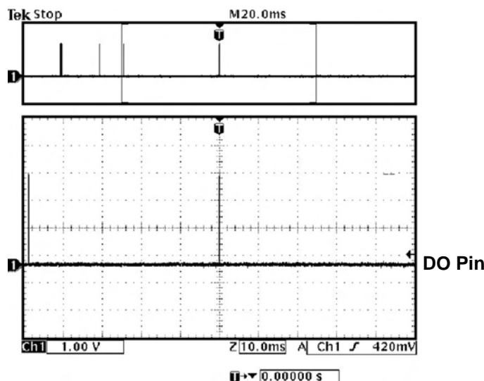
Figure 9. Data Out Pin with Squelch (SQ = 0)
